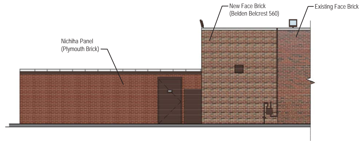
02 NORTH ELEVATION
