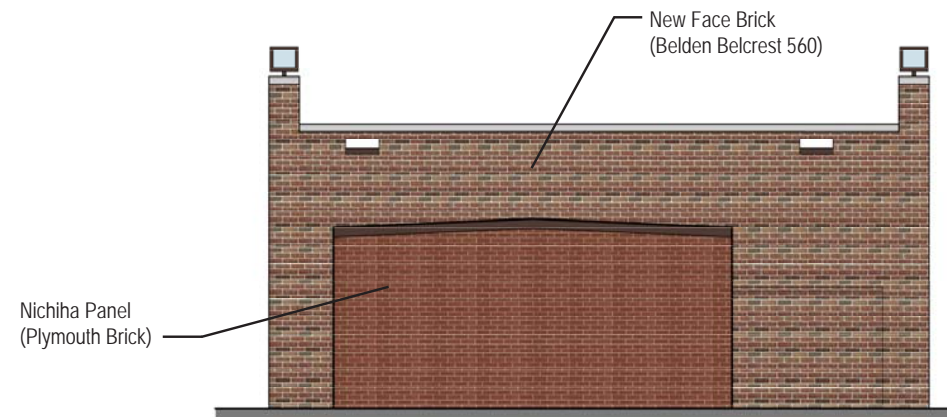
03 EAST ELEVATION
