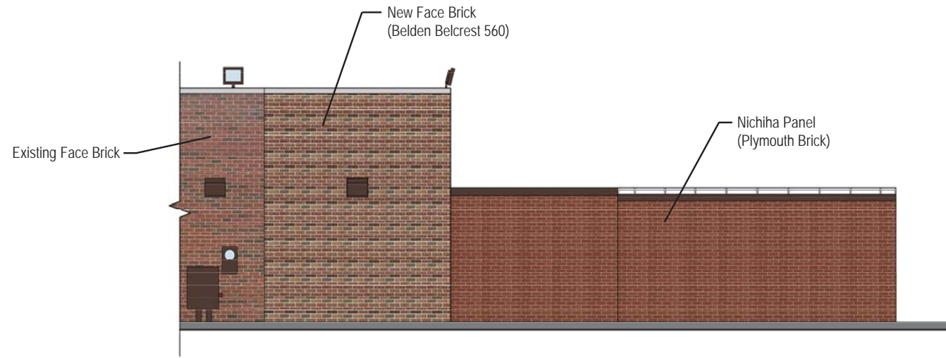
01 SOUTH ELEVATION
